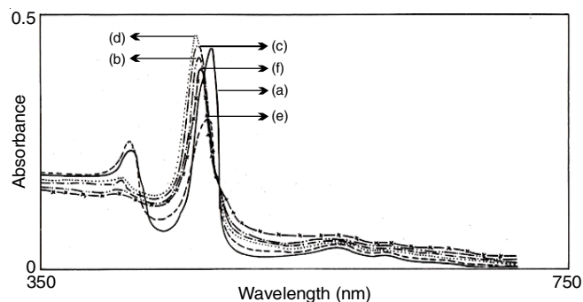
Fig. 6. Absorption spectra of \text{Mn(Py)}_4\text{P} with varying \text{SbCl}_5 concentration in \text{CH}_2\text{Cl}_2 recorded at ambient temperature
