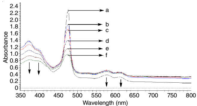
Fig. 5. Absorption spectra of 10^{-3} M \text{Mn(Py)}_4\text{P} with varying 2-methylimidazole concentration
