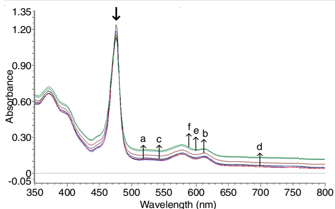
Fig. 4. Absorption spectra of 10^{-3} M \text{Mn(Py)}_4\text{P} with varying imidazole concentration
