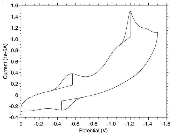
Fig. 2. Cyclic voltammogram of the mixture of 0.5 \times 10^{-3} M Mn(Py) 4 P and 0.1 M TBAP in dichloromethane recorded at room temperature with a 0.06 V/s scan rate
