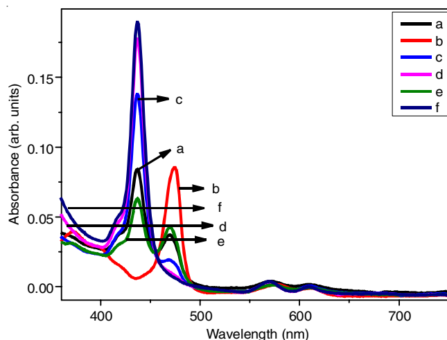
Fig. 3. UV-visible spectra of Mn(Py) 4 P with varying primary amine concentrations in dichloromethane recorded at room temperature
