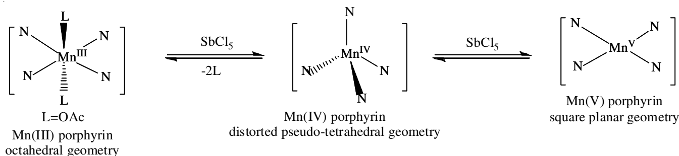
Scheme-I: Manganese(III) meso porphyrin converted to manganese(V) meso porphyrin through manganese(IV) meso porphyrin
