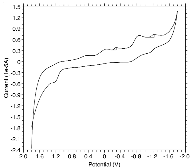
Fig. 1. Cyclic voltammogram of the mixture of 0.5 \times 10^{-3} M \text{Mn}(\text{Py})_4\text{P} and 0.1 M TBAP in dichloromethane recorded at room temperature with a 0.01 V/s scan rate
